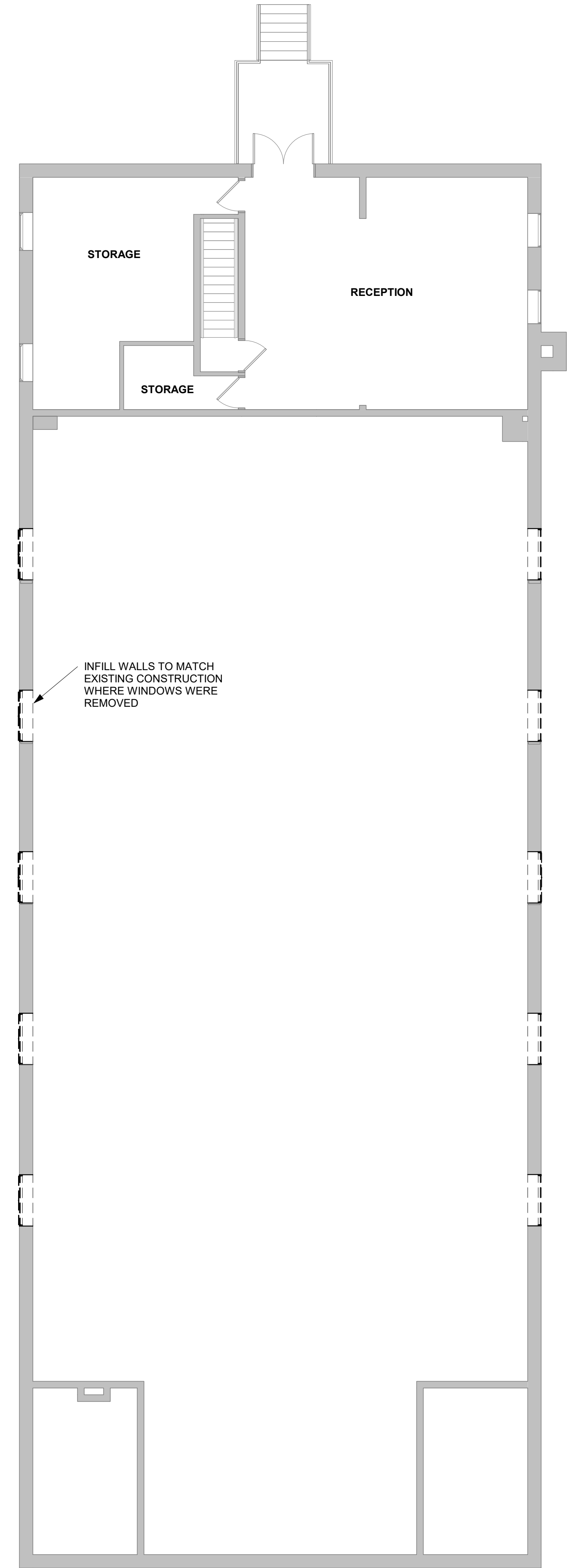
3 GYM - 2ND FLOOR - NEW WORK 1/8" = 1'-0"
