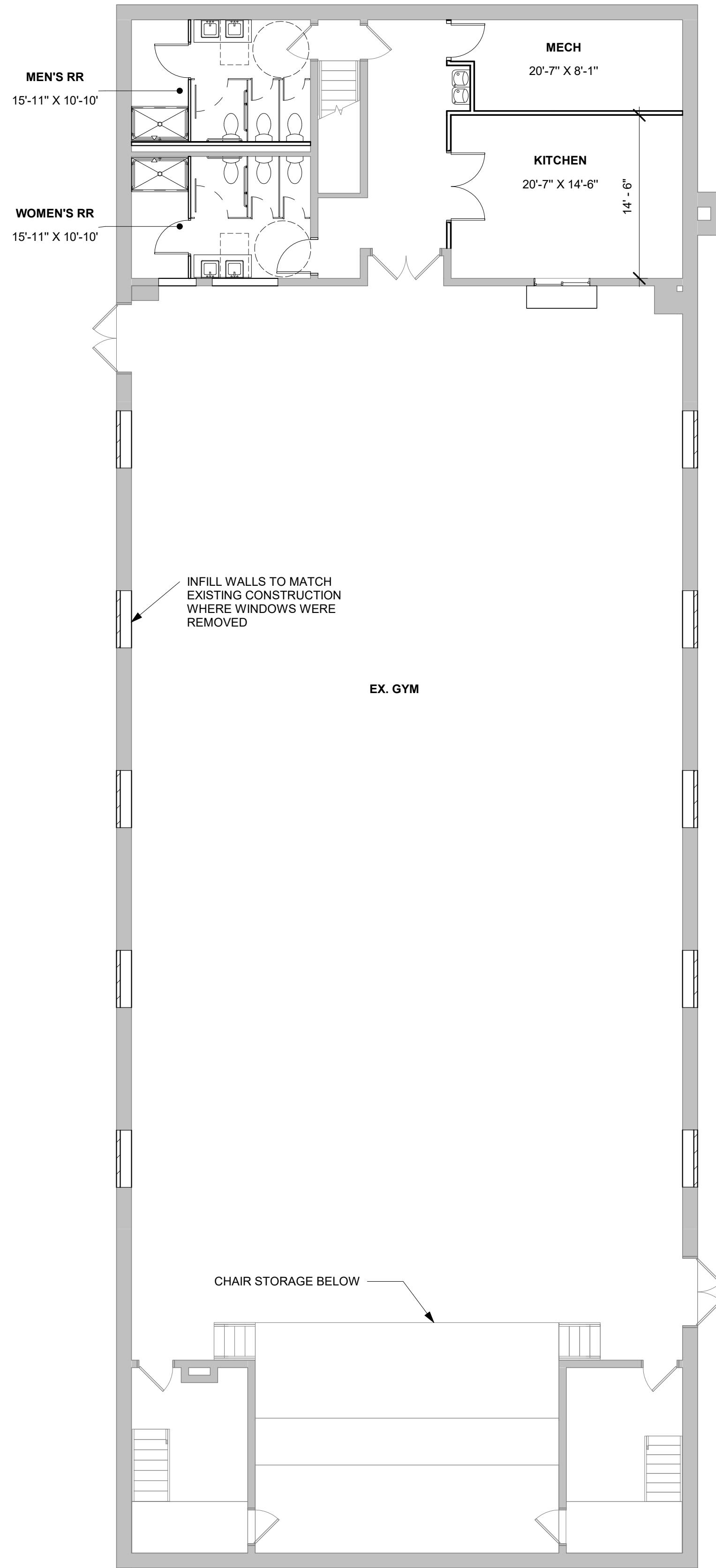
2 GYM - 1ST FLOOR - NEW WORK 1/8" = 1'-0"
